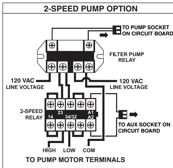
EasyTouch or IntelliTouch Load/Power Center
