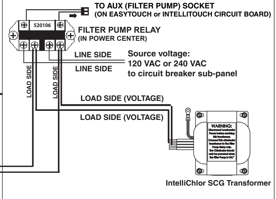
EasyTouch or IntelliTouch Load/Power Center
