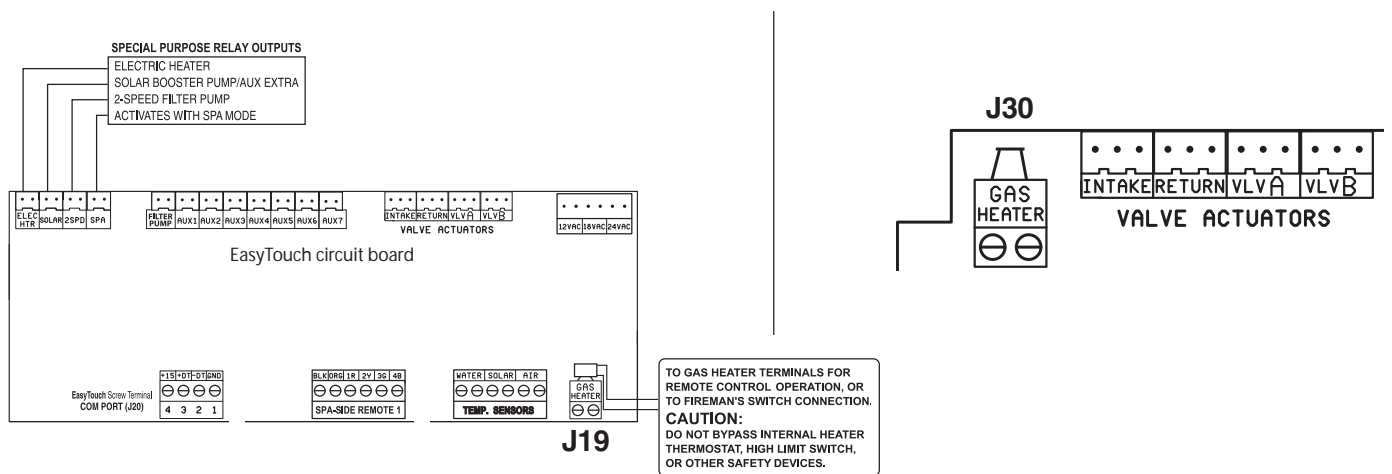
EasyTouch Circuit Board
