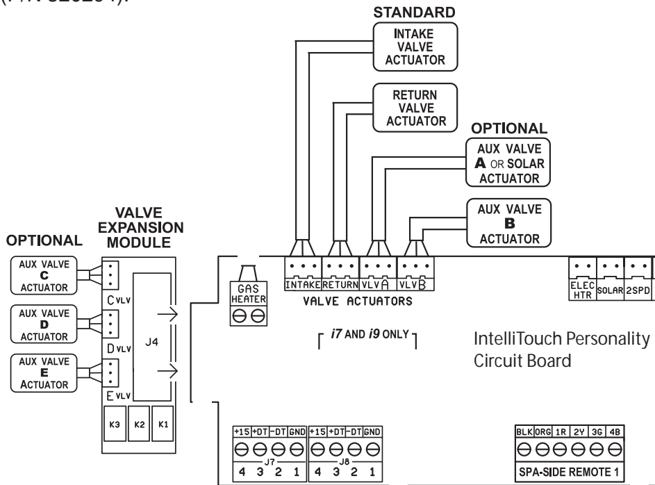
IntelliTouch Personality Circuit Board
